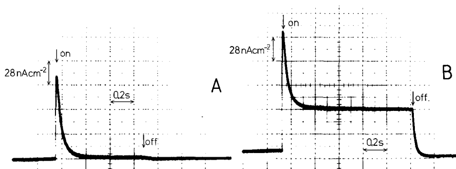
Fig. 1. Short-circuit photocurrent after addition of purple membrane fragments to one aqueous compartment. The aqueous phase contained 0.1 M \text{MgCl}_2 and 0.5 mM Tris, pH 7.0. The light was filtered through a K4 filter (Balzers, \lambda_{\text{max}} \approx 550 nm), yielding a light intensity in the plane of the membrane of about 5.0 \text{ mW cm}^{-2} . The area of the black film was 1.8 \text{ mm}^2 . A: Photocurrent in the absence of gramicidin. The sign of the photocurrent corresponds to a proton transfer toward the bacteriorhodopsin-free side. B: After addition of 30 nM gramicidin A to the bacteriorhodopsin-free compartment. After switching off the light the current falls to a slightly negative value and approaches zero level (horizontal trace at left) within a few seconds. The record was made about 30 min after the addition of gramicidin; the higher amplitude of the initial current I_0 in record B as compared with record A is presumably due to the binding of additional purple membrane during this time (a similar increase of I_0 is observed in the absence of gramicidin). The dark conductance of the membrane after addition of gramicidin was about 10 \text{ nS cm}^{-2} .
