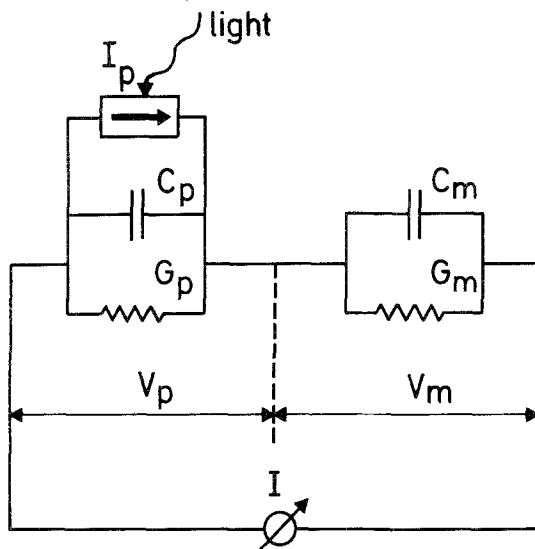
Fig. 5. Equivalent circuit of the model shown in Figure 4. G_p and C_p are the conductance and capacitance of the purple membrane; G_m and C_m are the corresponding values of the underlying part of the black film. Under short-circuit conditions the uncovered areas of the black film can be omitted from the equivalent circuit
