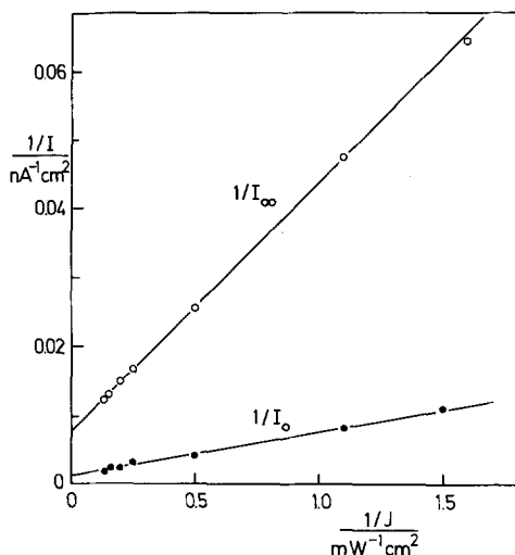
Fig. 3. Reciprocal values of the initial current I_0 (which is measured after switching on the light) and of the stationary current I_\infty as a function of reciprocal light intensity J . White light was filtered with a Balzers K4 filter ( \lambda_{\max} \simeq 550 \text{ nm} ), the light intensity was varied with a series of calibrated grey filters. All measurements have been performed with the same membrane in the presence of 30 nM gramicidin A; the aqueous phases contained 0.1 M \text{MgCl}_2 and 0.5 mM Tris, pH 7.0
