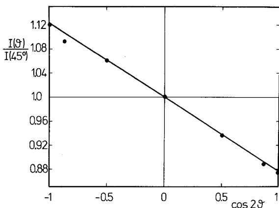
Fig. 9. Photoelectric effect with linearly polarized light. I(\theta) is the steady-state photocurrent ( I_\infty ) at low light intensity ( 0.05 \text{ mW cm}^{-2} ) and \theta is the angle between the electrical vector of the light and the plane of incidence (Fig. 8). The light was filtered through a Balzers K4 filter ( \lambda_{\text{max}} \approx 550 \text{ nm} ). To avoid light scattering in the cuvette, the light beam was focussed and centered on the membrane plane. The diameter of the light beam was about 0.8 mm, whereas the membrane diameter was 1.8 mm. \theta was varied by rotating the polaroid filter which was interposed between light source and membrane. The aqueous solutions contained 0.1 M \text{MgCl}_2 and 0.5 mM Tris, pH 7.0. 30 nM gramicidin A was added to the bacteriorhodopsin-free compartment. The level of the aqueous phases on both sides of the membrane was carefully controlled in order to keep the membrane planar. The experimental data were corrected for the residual polarization of the light source and the optical system in the following way. The membrane was replaced by a bolometer and the bolometer signal S(\theta) was measured as a function of the rotation angle \theta of the polaroid filter. The ratio I(\theta)/I(45^\circ) was corrected by multiplying the measured value of I(\theta)/I(45^\circ) by the factor S(45^\circ)/S(\theta) . The correction was opposite to the polarization effect on the photocurrent and the deviation of S(45^\circ)/S(\theta) from unity was less than 0.06. I(\theta) was symmetrical with respect to \theta = 0 within the limits of experimental error; the data points represent the average of I(+\theta) and I(-\theta) .
